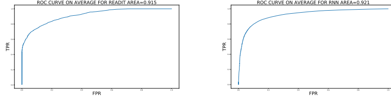
Fig. 2. On left the average ROC curve obtained by the mean of ROC curves out K iterations for READIT with AUROC=0.915. On right the average ROC curve obtained by the mean of ROC curves out K iterations for RNN with AUROC=0.921.
