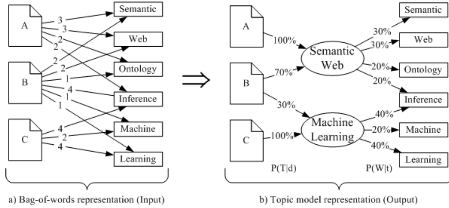
Fig. 1. The given corpus in bag-of-words format (a) is represented by a topic model (b) with mixing proportions of topics in documents P(T|d) and words in topics P(W|t) . Document A and C are only about one topic, whereas document B is about both the topics Semantic Web and Machine Learning, with a stronger focus on Semantic Web. The significant words for the both topics are very distinct, but the term “Inference” is used in both topics.
