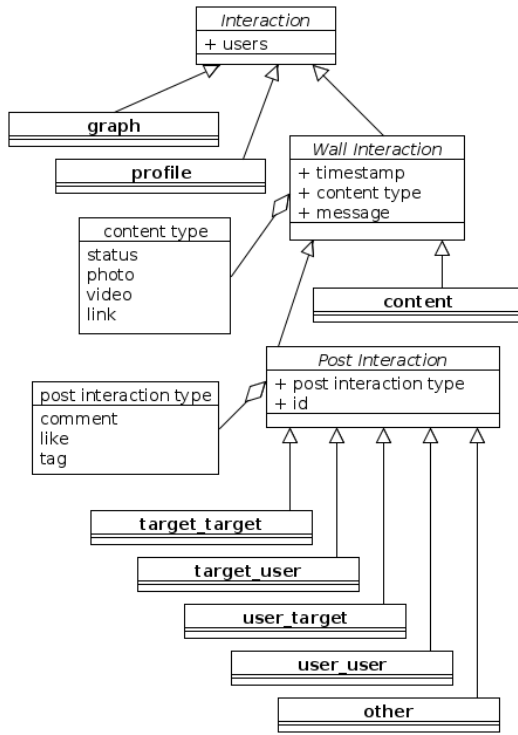
Figure 1: The hierarchy of interaction types
