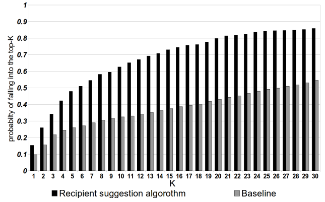
Figure 4: The probability for a user selected by expert to fall into top-K users. Recipient suggestion and Baseline algorithms
