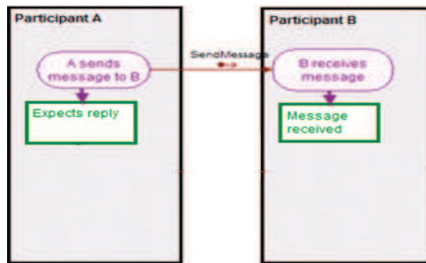
Fig. 2 BORM Diagram of Process A after Basic UCBA Transition
